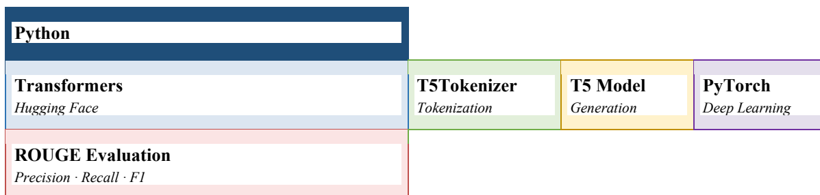
Figure 3.2: Technology Architecture
