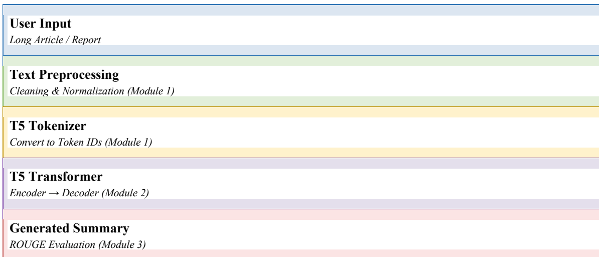
Figure 3.3: System Architecture
